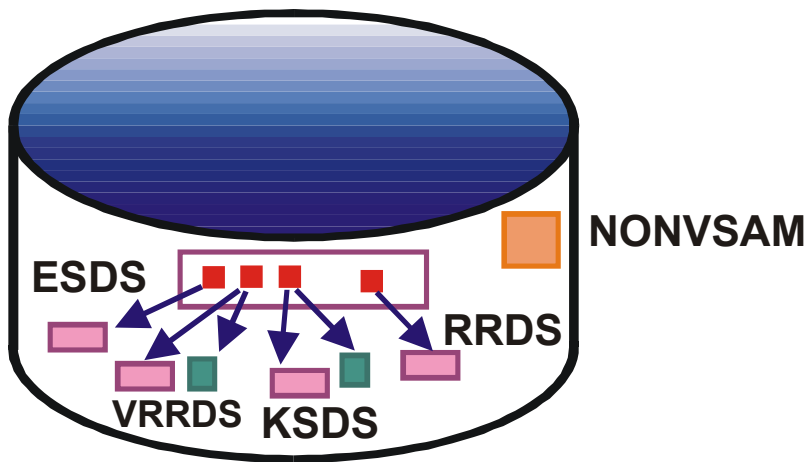
VSAM and non-VSAM datasets can reside on the same disk
